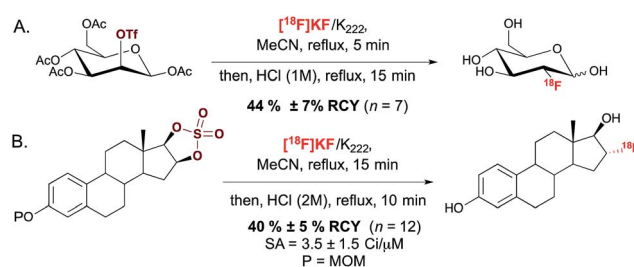
Scheme 1 (A.) Radiosynthesis of 2-[ 18 F]fluoro-2-deoxy-D-glucose ([ 18 F]FDG). (B.) Radiosynthesis of 16- \alpha -[ 18 F]fluoroestradiol ([ 18 F]FES). SA = specific activity. MOM = methoxymethyl.
