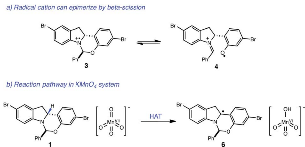
Fig. 3 (a) Proposed pathway for epimerization of starting material. (b) Proposed mechanism for \text{KMnO}_4 -mediated oxidation of indoline core.
