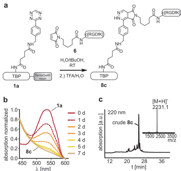
Fig. 6 \text{DAR}_{\text{inv}} on resin with \text{c(RGDfK(maleimide))} . (a) Reaction scheme of the \text{DAR}_{\text{inv}} . The tetrazine bearing resin was incubated with the diene 6 dissolved in \text{H}_2\text{O}/\text{tBuOH} . The peptide product was cleaved off from the resin by TFA. (b) Absorption scan of resin bound tetrazine 1a during the \text{DAR}_{\text{inv}} to monitor the progress of the reaction. (c) Crude RP-HPLC chromatogram and MALDI-ToF MS of the \text{DAR}_{\text{inv}} product 8c .
