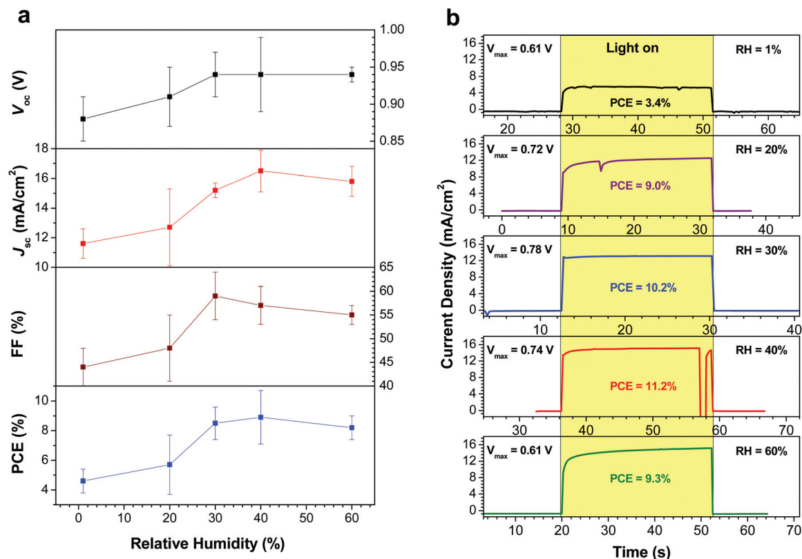
Fig. 6 (a) Average device performance characteristics (measured at a scan rate of 0.1 V s -1 ) as a function of relative humidity. Error bars represent plus or minus one standard deviation from the mean. (b) Steady-state current densities for representative devices at each relative humidity.
