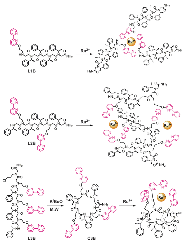
Fig. 1 Chemical structures of peptoid oligomers bearing 2,2'-bipyridine units and their anticipated ruthenium complexes.
