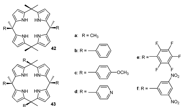
Fig. 22 Molecular structures of the calix[4]pyrrole-based anion receptors as used by Ballester's group for their quantification of anion- \pi interactions in solution. 46
