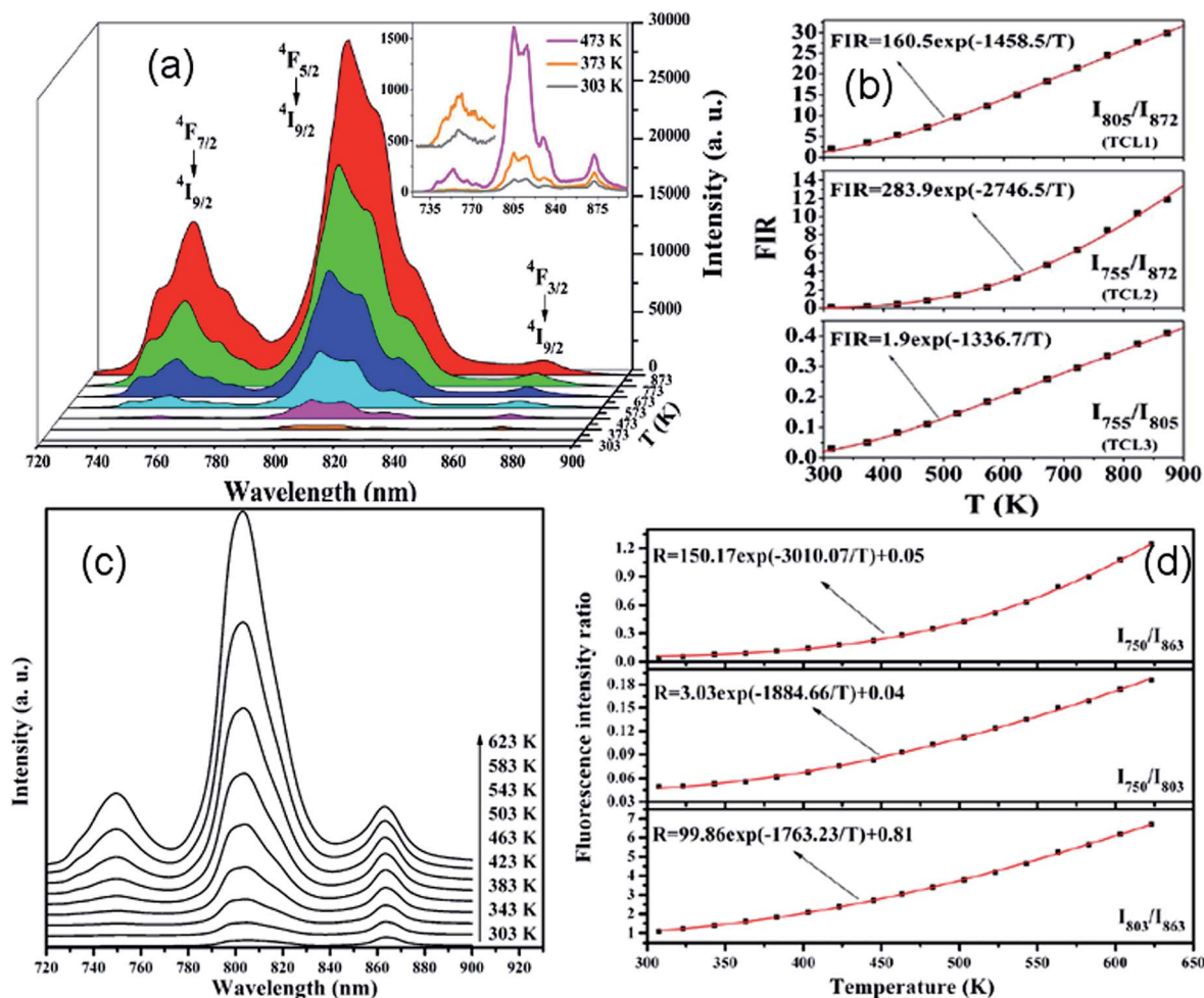
Fig. 13 Temperature dependent (a) near infrared emission spectra and (b) fluorescence intensity ratio (FIR) in Nd 3+ /Yb 3+ co-doped CaWO 4 phosphors excited by a 980 nm laser. Temperature dependent (c) near infrared emission spectra and (d) FIR in Nd 3+ /Yb 3+ co-doped oxyfluoride glass ceramic containing PbF 2 nanocrystals excited by a 980 nm laser. Reproduced from ref. 70 and 71 with permission of Optical Society of America and Elsevier.
