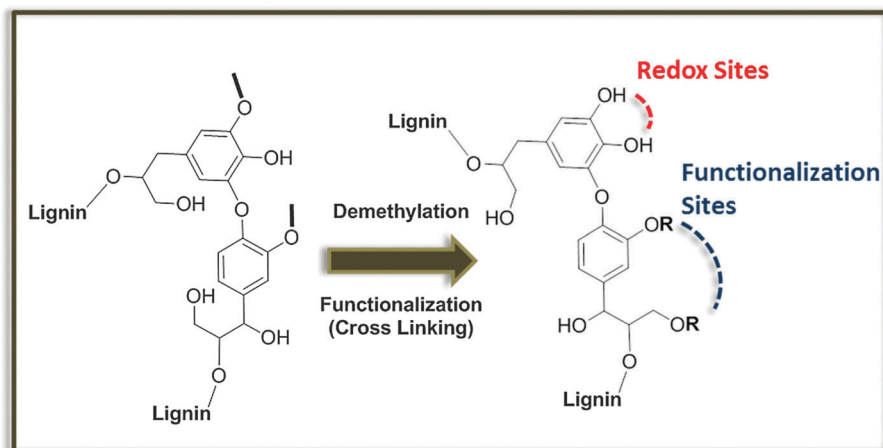
Fig. 9 Schematic aspects of the chemical modification of a lignin building block for its incorporation into polymers and materials.
