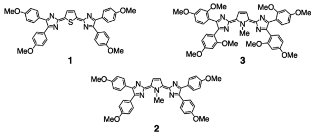
Fig. 1 Chemical structures of heterocyclic quinoid molecules 1–3 .
