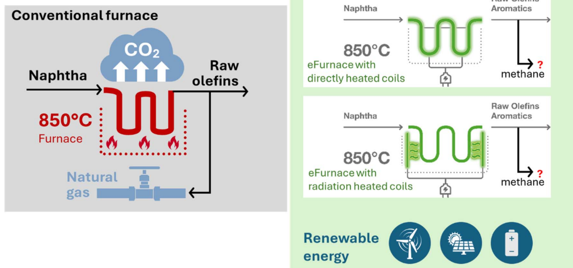
Fig. 17 A schematic comparison of the operation principle of a conventional steamcracker (left) and two versions of the eFurnace (right). Due to the electrically heated process, any methane formed in steam cracking that today is fed back as fuel for the process, will be available for other chemical raw material uses. (Source: BASF).
