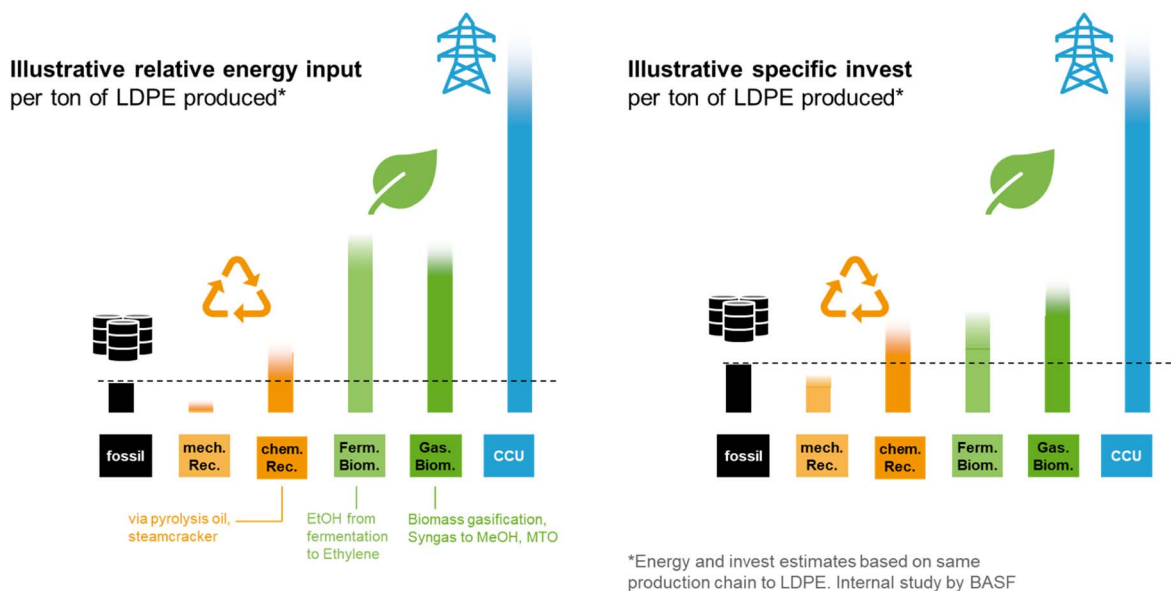
Fig. 19 Case study for different production routes to low density polyethylene (LDPE), a typical large-volume petrochemical product with a C : H ratio of ~1 : 2. The indicated energy input and invest volumes have been calculated for different raw-material routes: conventional fossil production, mechanical recycling (assuming equal quality can be achieved), chemical recycling via pyrolysis and naphtha replacement in the steam cracker (entry point 1 in Fig. 14), production via bio-ethanol from sugar fermentation to ethylene, waste biomass gasification, methanol synthesis and subsequent methanol-to-olefin (MTO) conversion (entry point 2 in Fig. 14), and finally CCU, namely captured CO 2 to methanol, and MTO. (Data is based on detailed calculations with non-public sources, and therefore shown on a relative scale also indicating major uncertainties due to different possible assumptions).
