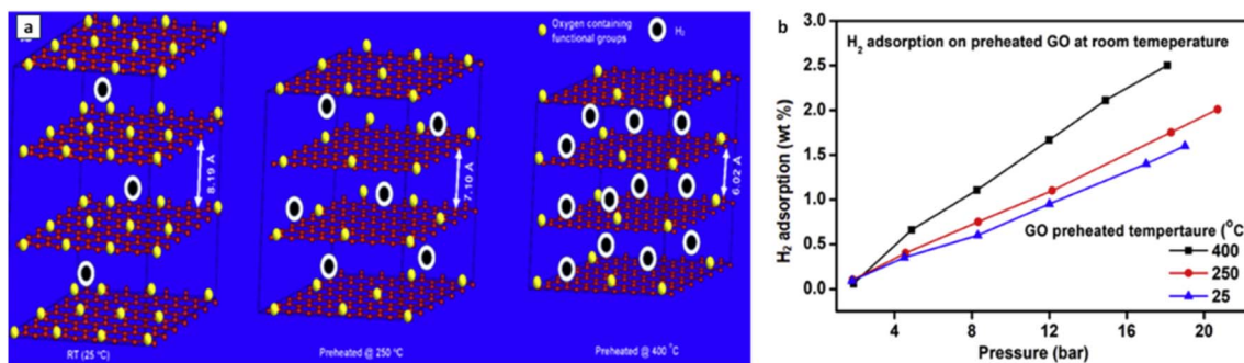
Fig. 5 The effect of interlayer distance of GO on \text{H}_2 adsorption (a) the control of interlayer spacing by altering the pretreatment temperature, (b) the \text{H}_2 adsorption properties of GO samples with different interlayer distances 77 (reproduced from ref. 77 with permission from Elsevier, copyright 2020).
