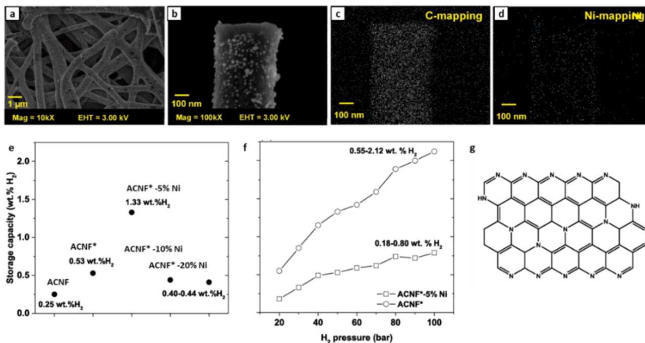
Fig. 6 Improving the \text{H}_2 adsorption of activated carbons via metallic nanoparticle decoration. (a–d) SEM images and EDX-mappings of 5 wt% Ni-doped ACNFs, (e and f) \text{H}_2 adsorptions at RT of ACNFs with and without Ni-doping with different Ni content, and (g) chemical structure of ACNF* 67 (reproduced from ref. 67 with permission from Elsevier, copyright 2021).
