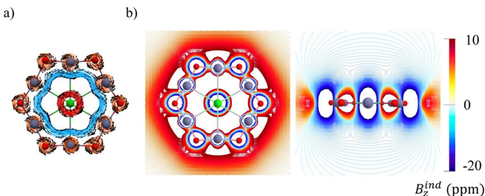
Fig. 4 (a) Magnetically induced current density J^{\text{ind}} maps for \text{Cl@Zn}_6\text{O}_6^- . Arrows indicate the direction of the current density. (b) B_z^{\text{ind}} isolines plotted in the molecular plane (bottom) and a transverse plane (top) of the \text{Cl@Zn}_6\text{O}_6^- . The external magnetic field is oriented perpendicular to the molecular plane.
