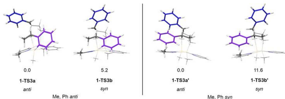
Fig. 11 The four isomeric model transition states studied. Values given are relative Gibbs free energies in kJ mol -1 . Absolute stereochemistry is labelled according to the relation between Me on catalyst and Ph on chain (purple) in the conformation when H projects into other chain.
