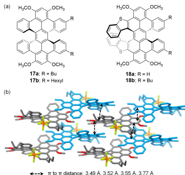
Fig. 6 (a) Double helicenes 17a/b and 18a/b ; (b) \pi – \pi stacking in the crystal of 17a^{+\bullet}PF_6^- , where the (M, M) enantiomer is shown in blue, and the (P, P) enantiomer is colored according to the elements. Reproduced with permission from ref. 40. Copyright 2022 American Chemical Society.
