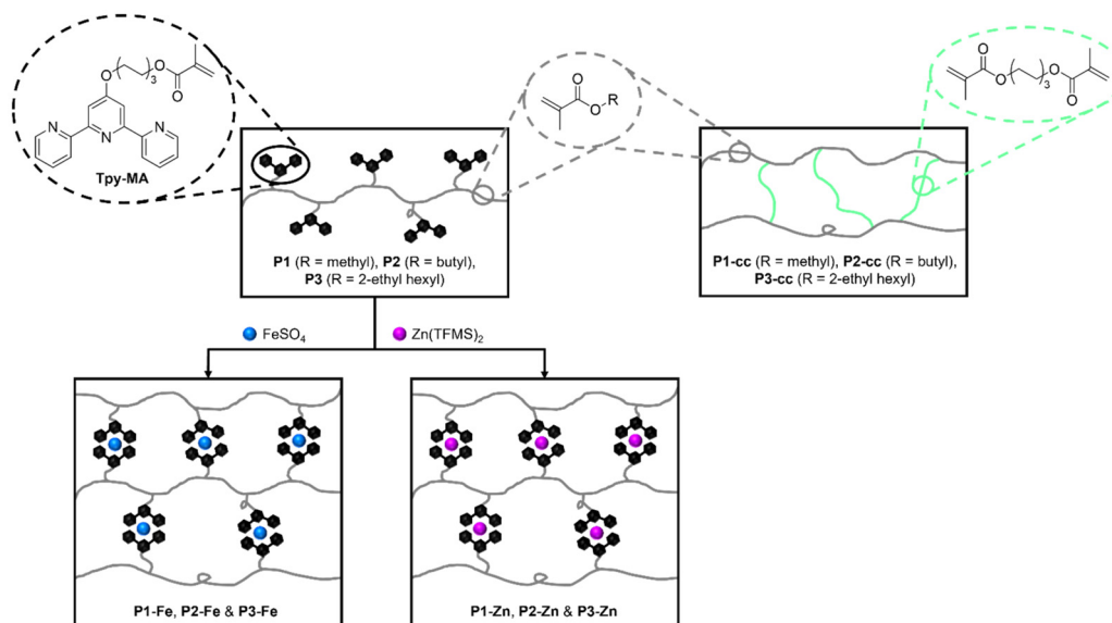
Scheme 1 Schematic representation of the synthesis of all metallopolymer networks P1-Fe to P3-Zn and of the polymer networks P1-cc to P3-cc.
