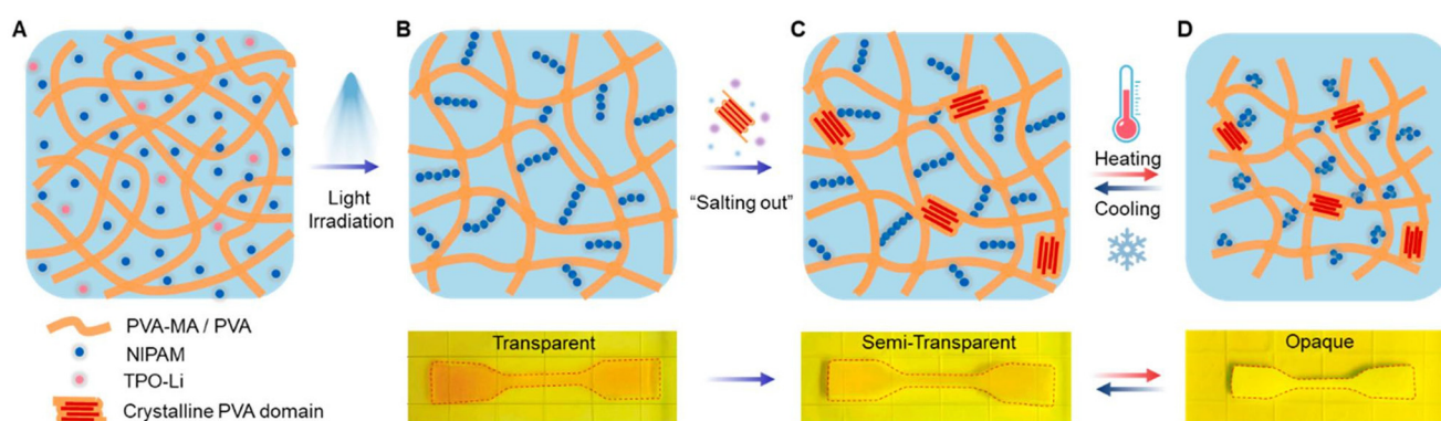
Fig. 3 Illustration of heating and cooling of PVA/(PVA-MA)- g -PNIPAM hydrogel. (A) Aqueous precursor containing PVA, PVA-MA, NIPAM and TPO-Li. (B) One-pot synthesis of PVA/(PVA-MA)- g -PNIPAM hydrogel by light irradiation from a digital light processing 3D printer. The as-printed hydrogel was transparent. (C) Toughening of hydrogel by immersion in Na 2 SO 4 salt solution to induce PVA aggregation and crystallization. The hydrogel turned semitransparent after the salting-out process. Upon heating, the hydrogel is actuated, turning into its coiled state represented in (D). The hydrogel turned completely opaque in this state after heating, and reverted back to its semitransparent state (C) after cooling. Reprinted and modified with permission from ref. 59, ACS, 2021.
