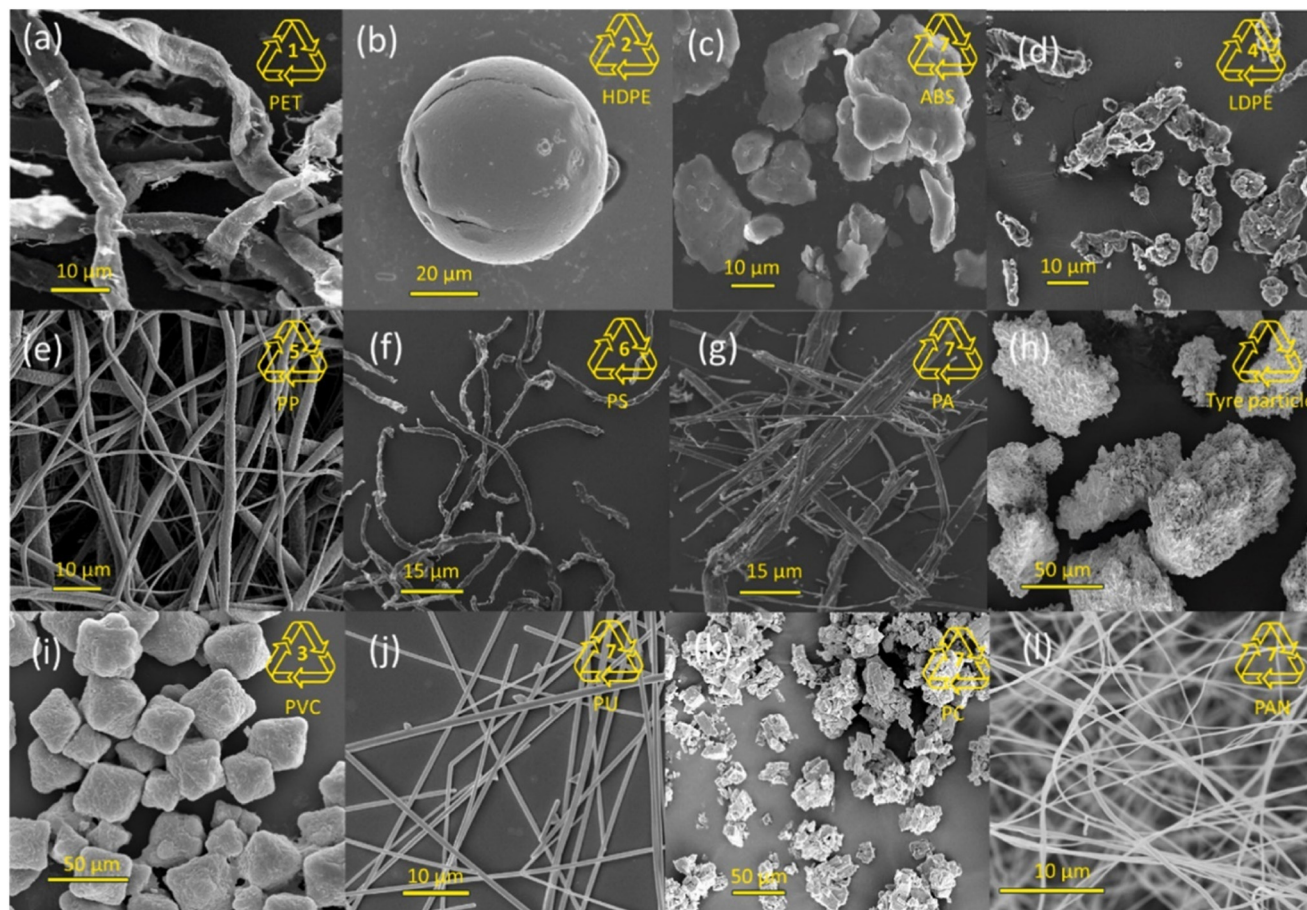
Fig. 4 (a) PET microfibers from the kitchen towel, b) HDPE microbeads from the facial scrub cosmetics, c) ABS microplastic debris from children toys, d) LDPE microplastic debris from waste soft plastics due to aging, e) PP microplastic fibers debris from kitchen scrubber, f) PS microfibers from textiles, g) PA microfibers from fabric, h) rubber Tyre debris, i) laboratory generated PVC microplastics, j) PU microfibers used to produce synthetic leather, k) PC debris from the fractured headlamp of old cars, and l) PAN precursor nanofiber. Authors own the analysis and characterisation.
