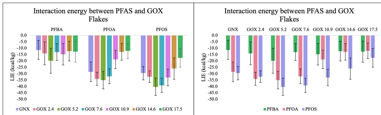
Fig. 2 Linear interaction energy between the PFAS and GOX flakes. Left panel – data is sorted by PFAS. Right panel – data is sorted by graphene oxide. All LIEs are given in kcal kg -1 of PFAS.
