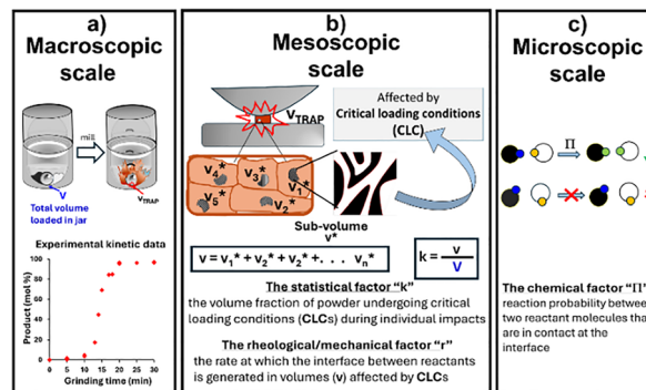
Fig. 51 Multiscale view of mechanochemical reactions. (a) Macroscopic scale: Powder ( V ) in the milling jar contains a small, trapped volume ( V_{trap} ) compressed between the ball and jar. Only global processes are observable. (b) Mesoscopic scale: forces in V_{trap} are unevenly distributed, creating sub-volumes ( v^* ). Only regions reaching "critical loading conditions" (CLC) undergo partial transformation, forming new interfaces between reagents (black and white). Parameters k and r are used in the kinetic model. (c) Microscopic scale: individual molecules react with probability \Pi , depending on orientation and chemical properties; \Pi is the third parameter in the kinetic model. 73
