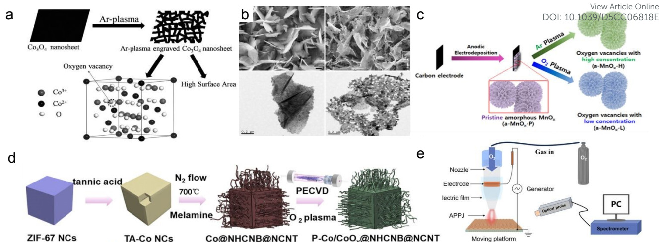
Figure 4 (a) Fabrication of oxygen-vacancy-rich \text{Co}_3\text{O}_4 with high surface area via Ar plasma engraving. (b) SEM and TEM images of pristine (left) and Ar-plasma engraved (right) \text{Co}_3\text{O}_4 , respectively. Reproduced with permission. 2 Copyright 2016, Wiley-VCH. (c) Schematic of the plasma treatment for the a- \text{MnO}_x catalysts with different concentrations of oxygen vacancies. Reproduced with permission. 17 Copyright 2020, Elsevier. (d) The synthesis process of the P-Co/ \text{CoO}_x @NHCNB@NCNT. Reproduced under the terms of CC-BY 4.0 license. 21 (e) Schematic illustration showing the APPJ setup and the treatment of the \text{MnO}_x film. Reproduced with permission. 32 Copyright 2024, Wiley-VCH.
