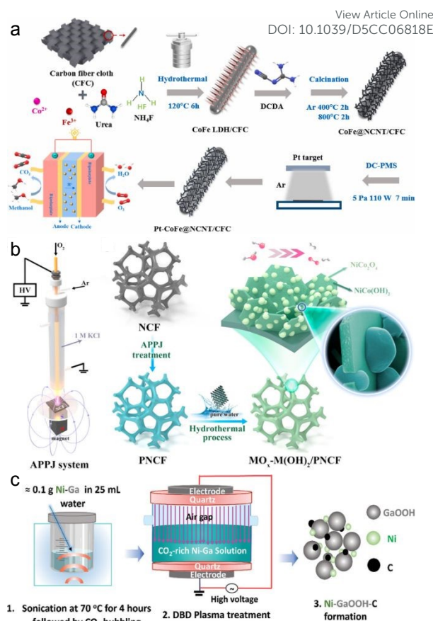
Figure 7 (a) Schematic illustration of the synthesis process of Pt–CoFe@NCNT/CFC electrode. Reproduced with permission. 7 Copyright 2022, Elsevier. (b) The schematic illustration for the fabrication of the electrode-emerged nanointerfaced bimetallic NiCo hydroxide–oxide active system. Reproduced with permission. 19 Copyright 2021, American Chemical Society. (c) Schematic showing the synthesis of Ni-GaOOH-C catalyst. Reproduced under the terms of CC-BY 4.0 license. 24
