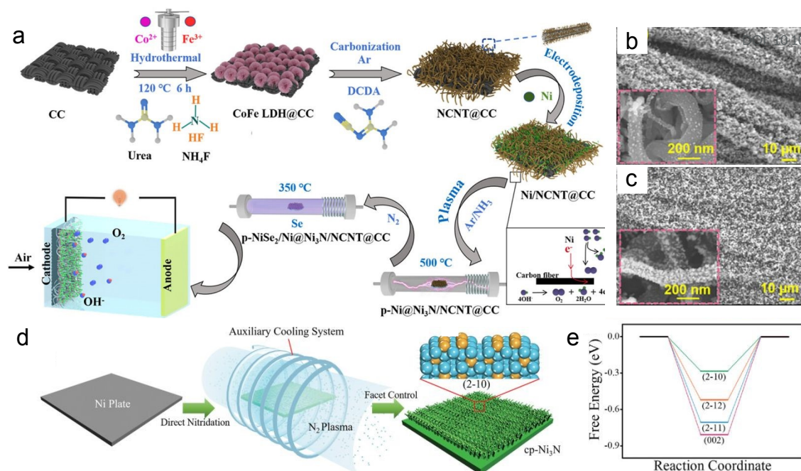
Figure 2 (a) Schematic illustration of the synthetic process of the p-NiSe 2 /Ni@Ni 3 N/NCNT@CC. SEM images of (b) p-Ni@Ni 3 N/NCNT@CC and (c) p-NiSe 2 /Ni@Ni 3 N/NCNT@CC. Reproduced with permission. 1 Copyright 2025, Wiley-VCH. (d) Schematic Illustration of the as-prepared Ni 3 N nano-frameworks through cooling-assisted plasma process. (e) Free energy for HER on typical facets of hexagonal Ni 3 N model. Reproduced with permission. 14 Copyright 2022, Wiley-VCH.
