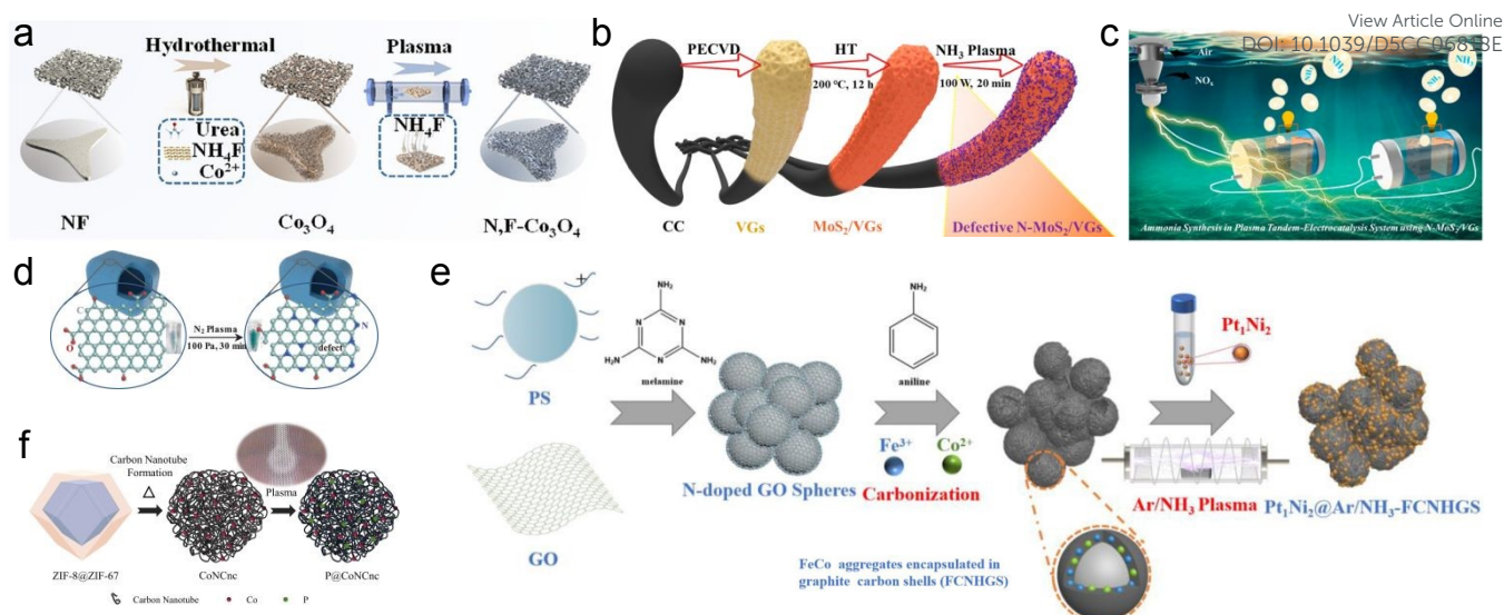
Figure 6 (a) Schematic illustration of the synthesis process of the N, F- \text{Co}_3\text{O}_4 . Reproduced with permission. 4 Copyright 2025, Wiley-VCH. (b) Schematic illustration for N- \text{MoS}_2/\text{VGs} engraved by RF \text{NH}_3 plasma. (c) The plasma tandem-electrolysis system. Reproduced under the terms of CC-BY 4.0 license. 8,9 (d) Schematic illustration showing the synthesis of N-doped quasi-graphene by \text{N}_2 Plasma. Reproduced with permission. 16 Copyright 2020, American Chemical Society. (e) Illustration of the fabrication of \text{Pt}_3\text{Ni}_2@Ar/\text{NH}_3\text{-FCNHGS} . Reproduced with permission. 29 Copyright 2023, Elsevier. (f) Schematic showing the P soft doping of CoNCnc by microwave plasma. Reproduced with permission. 34 Copyright 2025, Elsevier.
