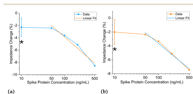
Fig. 4 Sensing of spike protein in saliva with antibody in 1 \times PBS solution. (a) Titration curve using updated data analysis method for SARS-CoV-2 spike proteins in saliva and antibodies in 1 \times PBS with 50–500 \text{ng mL}^{-1} dynamic range and 200 \text{ng mL}^{-1} (1.5 nM) detection limit; linear fit: (Z) = 8.36 - 6.11 \times (C) , R -square = 0.97. (b) Titration curve using previous data analysis method for SARS-CoV-2 spike proteins in saliva and antibodies in 1 \times PBS with 50–500 \text{ng mL}^{-1} dynamic range and 200 \text{ng mL}^{-1} (1.5 nM) detection limit; linear fit: (Z) = 6.74 - 5.2 \times (C) , R -square = 0.99. * Denotes negative control ( C = 0 \text{ ng mL}^{-1} ) plotted at C = 10 \text{ ng mL}^{-1} for visualization purposes, N = 5 for C = 0 \text{ ng mL}^{-1} , N = 1 for all other concentrations.
