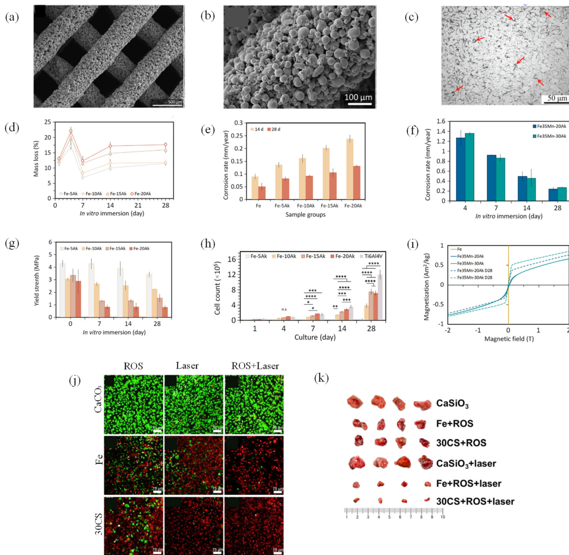
Fig. 6 Representative images of (a) the struts of the extrusion-based 3D printed Fe-Ak scaffolds 86 and (b) magnified image of the strut of Fe- 15 vol% Ak 86 and (c) SLM printed Fe-4Pd-5BR with red arrows pointing at BR. Graphical representation of the extrusion-based 3D printed scaffolds: (d) the mass losses of the Fe-xAk scaffolds through 28-day immersion in the r-SBF, 86 (e) corrosion rates determined from 14- and 28-day immersion testing, 86 (f) corrosion rates of the Fe35Mn-xAk scaffolds, 55 (g) yield strengths of Fe-xAk through 28-day immersion testing, 86 (h) cell count in preosteoblast culture for 28 days 86 and (i) magnetization curves of the FeMn-xAk specimens as-sintered and after in vitro degradation for 28 days. 55 (j) Images of the culture of Sao2 tumor cells with CaSiO 3 , Fe, and 30CS scaffolds treated with ROS, laser, and ROS + laser therapies and (k) images of tumors extracted on day 15 for each treatment and material. 172 (a, b, d, e, g and h) are reprinted from Elsevier, copyright 2022, licensed under CC BY 4.0; (c) is reproduced with permission from Elsevier, copyright 2019; (f and i) are reprinted from Elsevier, copyright 2023, licensed under CC BY 4.0; and (j and k) are reprinted from Nature, copyright 2018, licensed under CC BY 4.0.
