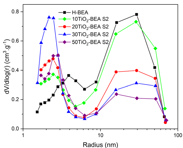
Fig. 4 Pore size distribution curves (BJH, desorption branch) of TiO 2 -BEA composites: (top) S1 series and (bottom) S2 series.
