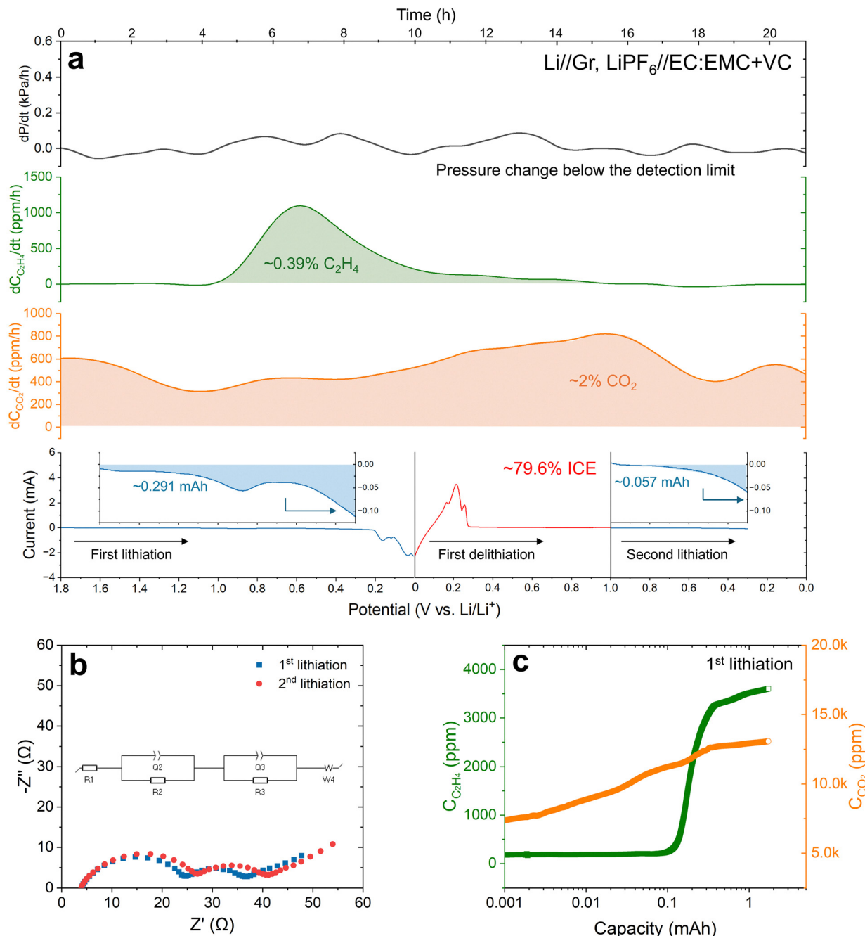
Fig. 7 Operando monitoring of gas evolution in the Li-graphite half-cell that undergoes cyclic voltammetry at a scan rate of 0.05 \text{ mV s}^{-1} with 1 \text{ M LiPF}_6 in EC:EMC 3:7 vol% + 2 vol% VC as the electrolyte. (a) The obtained CV curves are plotted in conjunction with the change in concentrations of \text{C}_2\text{H}_4 , \text{CO}_2 , and in overall gas pressure. The detailed current variation from 1.8 V to 0.3 V vs. \text{Li/Li}^+ of the first lithiation and from 1 V to 0.3 V vs. \text{Li/Li}^+ of the second lithiation is provided in the insets by zooming in the y-axis. The blue shading of the first lithiation represents the electric charge consumed for the SEI formation and associated gas evolution. (b) The EIS spectra obtained after the initial and the second cathodic scan. (c) Evolution of \text{C}_2\text{H}_4 and \text{CO}_2 concentrations during the initial lithiation of graphite.
