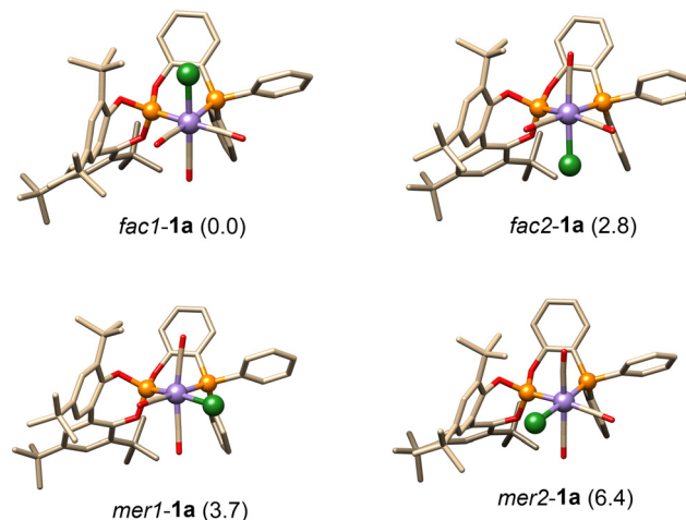
Fig. 5 Optimized geometries of isomers of 1a . Numerical values correspond to free energies relative to fac1 isomer (kcal \text{mol}^{-1} , hydrogens have been omitted for clarity).
