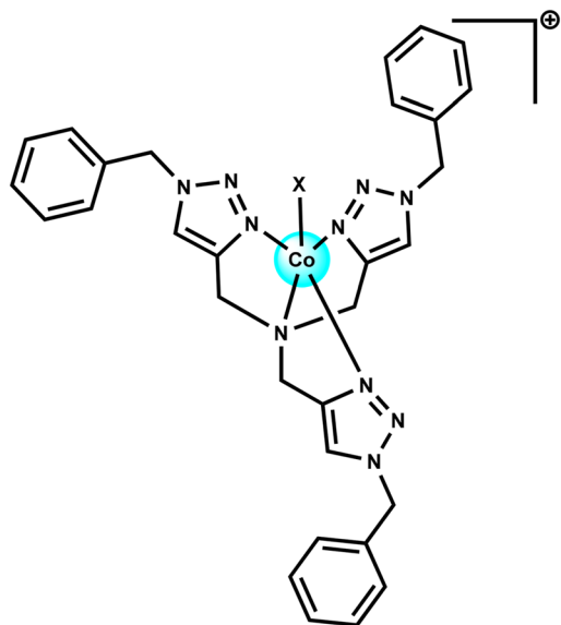
X = Cl; [Co(tbta)Cl](ClO 4 ); tbp, D = -7.5 \text{ cm}^{-1} . X = Br; [Co(tbta)Br](ClO 4 ); tbp, D = -4.3 \text{ cm}^{-1} . X = N 3 ; [Co(tbta)N 3 ](ClO 4 ); tbp, D = -10.7 \text{ cm}^{-1} .
