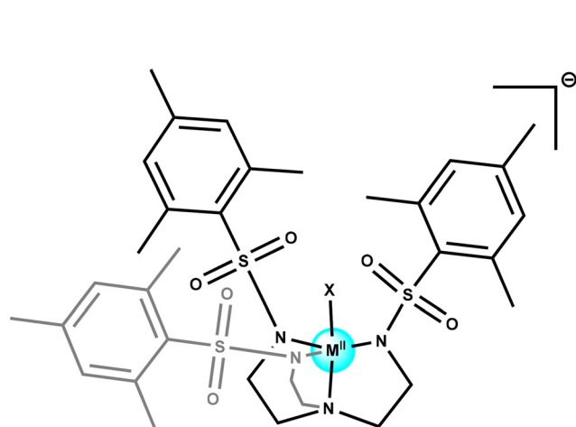
X = None, trigonal monopyramidal, [Co(MST)], D = 33 \text{ cm}^{-1} . X = OH 2 , [Co(MST)(OH 2 )], TBP, D = 24 \text{ cm}^{-1} . X = None, trigonal monopyramidal, [Fe(MST)], D = -31 \text{ cm}^{-1} . X = OH 2 , TBP, [Fe(MST)(OH 2 )], D = +8.7 \text{ cm}^{-1} . X = None, trigonal monopyramidal, [Ni(MST)], D = -276 \text{ cm}^{-1} . X = OH 2 , TBP, [Ni(MST)(OH 2 )], D = -209 \text{ cm}^{-1} .
