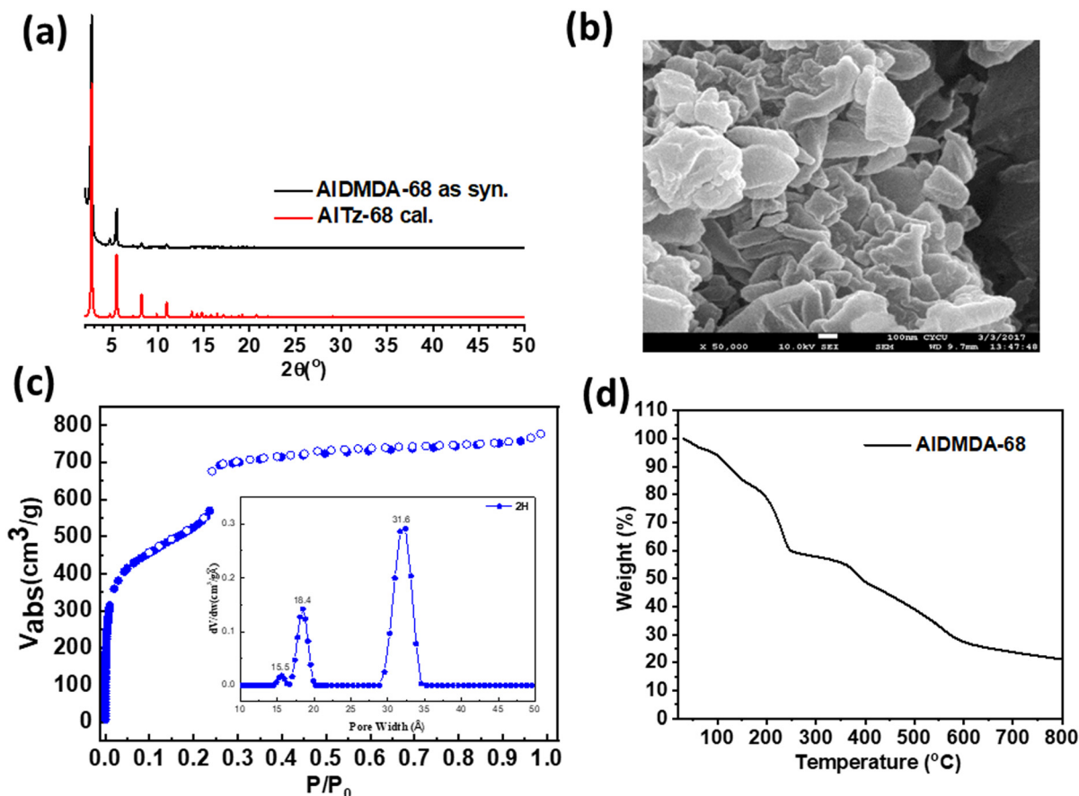
Fig. 2 (a) PXRD of AIDMDA-68. (b) SEM images of AIDMDA-68. (c) \text{N}_2 sorption isotherms of AIDMDA-68 (inset: pore size distribution of AIDMDA-68). (d) TGA curve of AIDMDA-68.
