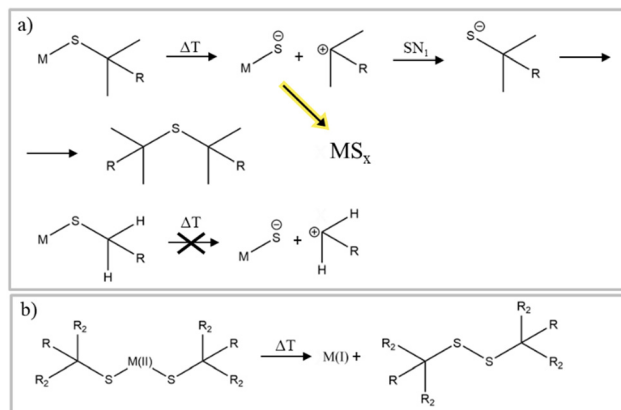
Fig. 4 (a) Thermal decomposition of thiolates and formation of MS x nanomaterials. Figure adapted from ref. 79 under Creative Commons Attribution licence CC BY 4.0 (b) redox reaction of thiolates and metals reported in ref. 86.
