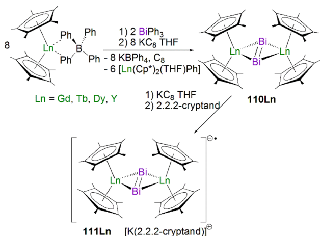
Scheme 35 Synthesis of lanthanide dibismuth complexes 110Ln – 111Ln .
