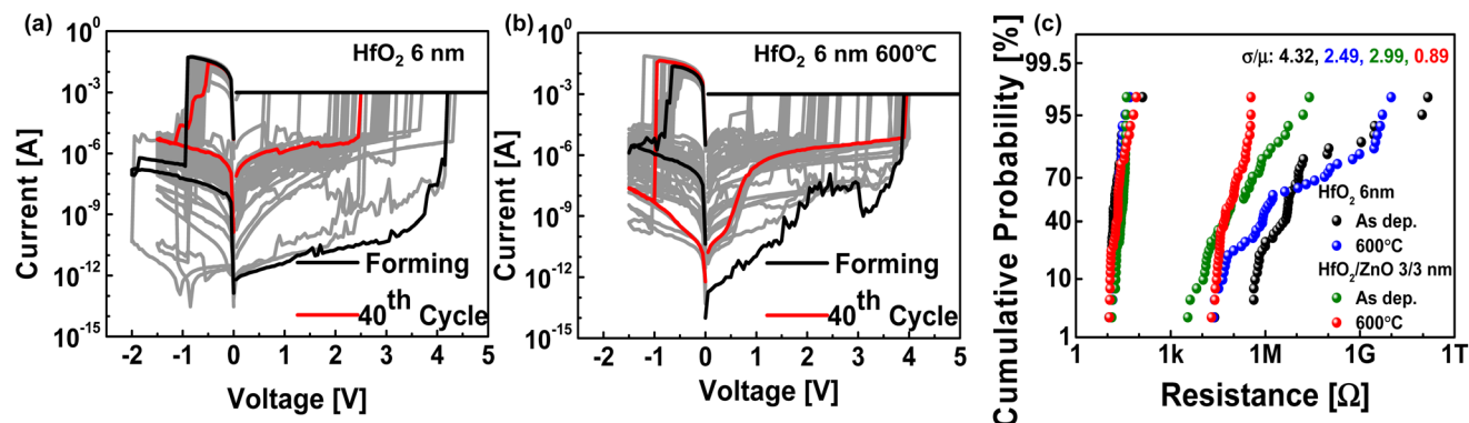
Fig. 7 Typical I - V switching behavior of 6 nm \text{HfO}_2 (a) without and with thermal annealing (b) at 600^\circ\text{C} for 1 h in an \text{N}_2 ambient compared with that of bilayer \text{HfO}_2/\text{ZnO} synaptic devices under the same thermal annealing conditions. (c) Distribution and cumulative probability of the HRS and LRS of \text{HfO}_2 (6 nm) and bilayer 3 nm \text{HfO}_2/3 nm \text{ZnO} synaptic devices without and with thermal annealing.
