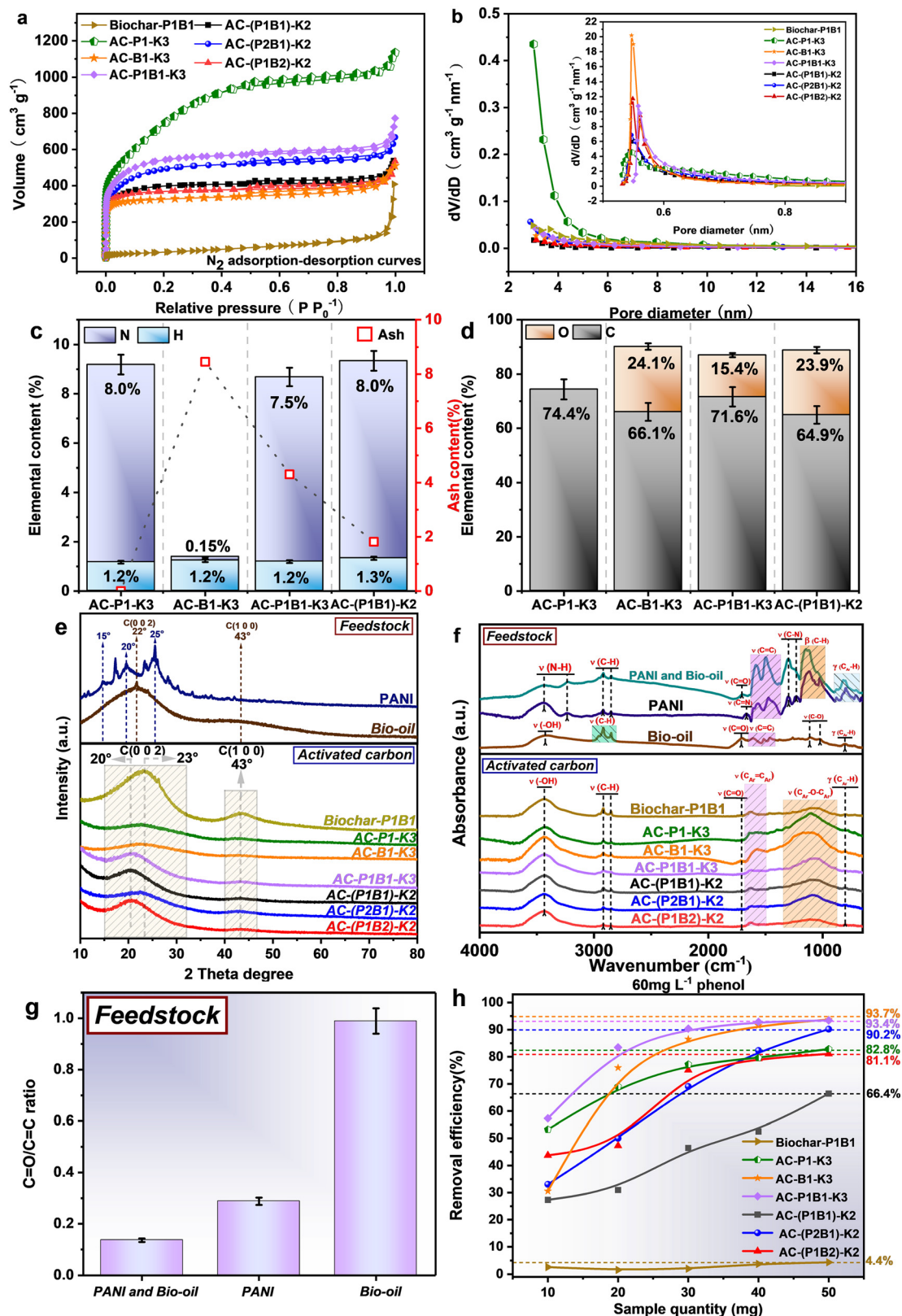
Fig. 3 Characterization of activated carbon; (a and b) Pore characteristics of the activated carbon; (c and d) elemental analysis of activated carbon (O = 100% - C% - H% - N% - S% - H 2 O% - ash%); (e) XRD characterization; (f) FT-IR characterization; (g) the C=O/C=C ratio of feedstocks in FT-IR characterization; (h) the removal efficiency of phenol by ACs.
