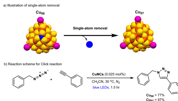
Fig. 5 Isostructural \text{Cu}_{57} NC & \text{Cu}_{58} NC catalyzed Click reactions.
