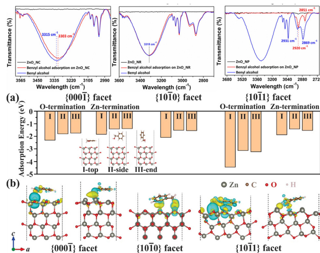
Fig. 10 IR absorption of different ZnO nanomaterial before and after BrnOH adsorption. The range is focused on the O–H stretch. (a) Calculated absorption energy of benzyl alcohol in different modes on different facets of ZnO hexagons. (b) Electron density prediction of varied facets of ZnO with adsorbed benzyl alcohol. Credit: H. Weerathunga, C. Tang, A. J. Brock, S. Sarina, T. Wang, Q. Liu, H. Y. Zhu, A. Du and E. R. Waclawik, J. Colloid Interface Sci. , 2022, 606 , 588–599.
