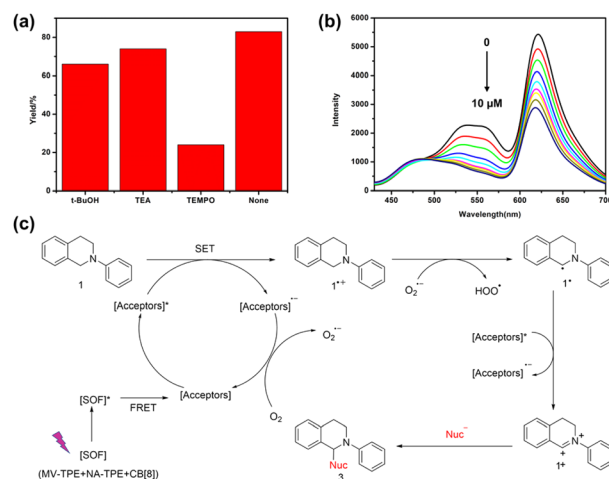
Fig. 4 (a) Control experiments of the CDC reaction in the presence of different scavengers: t\text{-BuOH} , TEA, and TEMPO. (b) Fluorescence emission spectra of the SOF + DBT + SR101 system in water with the addition of N -phenyl tetrahydroisoquinoline. (c) A plausible mechanism for the aerobic CDC reaction.
