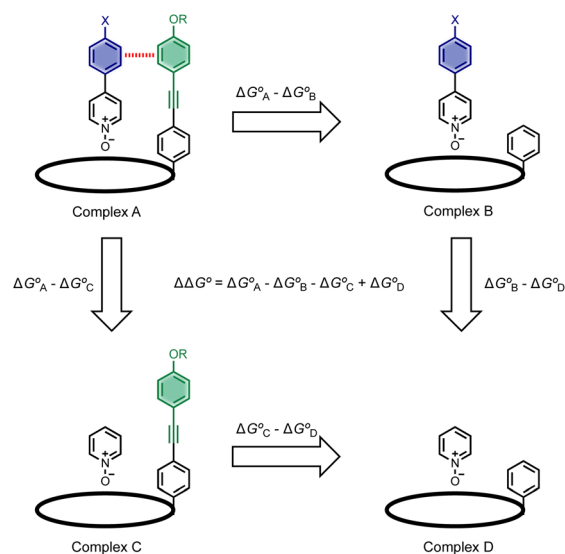
Fig. 2 Chemical double mutant cycle for evaluating the free energy contribution ( \Delta\Delta G^o ) due to aromatic interactions with the blue ring of the guest to the overall stability of complex A. Only one of the four calix[4]pyrrole side-arms is shown for clarity, but the DMC measures the sum of interactions with four green aromatic rings on the host.
