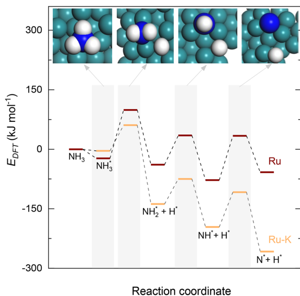
Fig. 3 Potential energy surface profile of the dehydrogenation of NH 3 ( y = 1-3 ) on Ru(111) and the corresponding transition states and Ru-K/CaO(111). The respective transition states of which are depicted in Fig. 4.
