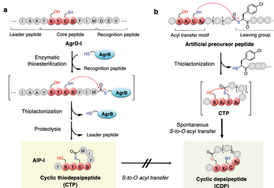
Fig. 1 Ribosomal synthesis of cyclic thiodepsipeptides (CTPs) possessing an SX_1CX_2 motif and a downstream thioester. (a) Biosynthesis of autoinducing peptide I (AIP-I) from AgrD-I as a precursor peptide. (b) One-pot in vitro ribosomal cyclic depsipeptide (CDP) synthesis. In this case a CTP acts as an intermediate and is spontaneously converted to CDP via an S-to-O acyl transfer modulated by an SX_1CX_2 motif. N \geq 1 , depending on the X_2 residue.
