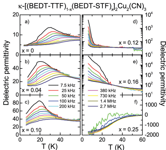
Fig. 8 The dielectric permittivity of \kappa -[(BEDT-TTF) _{1-x} (BEDT-STF) _x ] _2 Cu _2 (CN) _3 is shown for substitutions x = 0, 0.04, 0.10, 0.12, 0.16 and 0.25 as a function of temperature for different frequencies. (a–c) A relaxor-ferroelectric response is observed for the insulating compounds ( x \leq 0.10 ) below T = 50 K. Upon reducing the measurement frequency, the feature becomes more pronounced and shifts to lower temperatures. (d and e) As a result of coexistence of spatially separated metallic and insulating regions at the IMT, \epsilon_1 reaches values of 10^5 , with a pronounced frequency dependence. (f) Well above the percolation threshold, from x > 0.2 up to x = 1 , the dielectric constant acquires negative values for x > 0.2 as the sample turns metallic. Note the different ordinates of the various panels.
