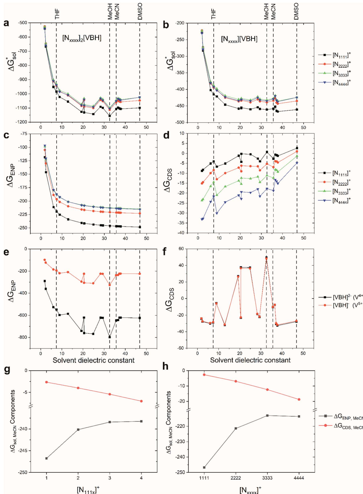
Fig. 5 Solvation free energies, \Delta G_{sol}^* , of VBH with the symmetric cations in its (a) reduced and (b) oxidized states. Also shown are the comprising bulk-electrostatic, \Delta G_{ENP} , and non-electrostatic, \Delta G_{CDS} , components of the solvation energies for each ion: panels (c) and (d) for the \Delta G_{ENP} and \Delta G_{CDS} of symmetric cations, respectively, while panels (e) and (f) for the VBH anion in the +4 and +5 oxidation states. Panels (g) and (h) show the changes in the \Delta G_{ENP} and \Delta G_{CDS} in MeCN as the alkyl chain lengths are increased for [N 111x ] + and [N xxxx ] + respectively. All energy values are in kJ mol -1 units.
