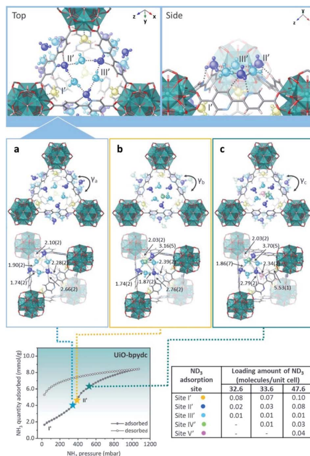
Fig. 22 (Top) Refined \text{ND}_3 positions in the UiO-bpydc structure at \text{ND}_3 loadings of (a) 4.15, (b) 4.27, and (c) 6.06 \text{mmol g}^{-1} obtained from NPD data at 300 K. (Bottom) \text{ND}_3 molecules at different binding sites: site I': yellow, site II': blue, site III': light blue, site IV': pink, and site V': green. \text{NH}_3 sorption isotherm at 298 K and up to 1100 mbar; adsorption: closed circles; desorption: open circles reprinted with permission from ref. 112. Copyright (2021) American Chemical Society.
