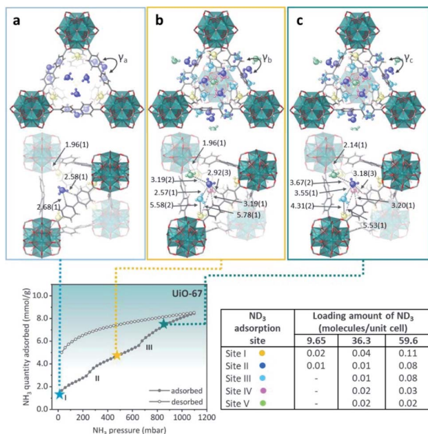
Fig. 21 (Top) Refined \text{ND}_3 positions in the UiO-67 structure at \text{ND}_3 loadings of (a) 1.23, (b) 4.63, and (c) 7.60 \text{mmol g}^{-1} obtained from NPD data at 300 K. \text{ND}_3 molecules at different binding sites: site I: yellow, site II: blue, site III: light blue, site IV: pink, and site V: green. (Bottom) \text{NH}_3 sorption isotherm at 298 K and up to 1100 mbar; adsorption: closed circles; desorption: open circles reprinted with permission from ref. 112. Copyright (2021) American Chemical Society.
