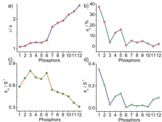
Phosphors: 1. PDNA-10, 2. PDNA, 3. 1,2-Oph-PLA, 4. PDNA-5, 5. 2-HC in PVA, 6. PVA-100-P4-1, 7. BDPB-Ac, 8. BDPB, 9. BP, 10. BDPD-PPT, 11. TAT, 12. CS
