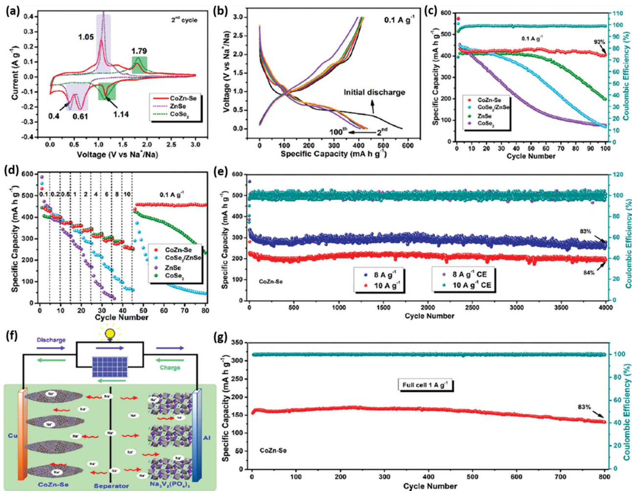
Fig. 7 \text{Na}^+ storage properties. (a) CV curves at the scan rate of 0.1 \text{ mV s}^{-1} for CoZn-Se, ZnSe, and CoSe 2 -based electrode materials. (b) Galvanostatic charge-discharge potential profiles at 0.1 \text{ A g}^{-1} of CoZn-Se. (c) Cycling performance at 0.1 \text{ A g}^{-1} . (d) Rate capability at various current densities of the electrode materials. (e) Cycling stability performance of CoZn-Se. (f) Schematic representation of the \text{Na}_3\text{V}_2(\text{PO}_4)_3|\text{CoZn-Se} full cell. (g) Cyclic stability at 1 \text{ A g}^{-1} of the full cell. Reprinted with permission from ref. 94. Copyright 2019 American Chemical Society.
