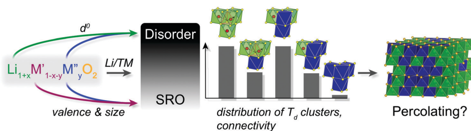
Fig. 9 Factors contributing to the stabilization of a DRX lithium transition metal oxide structure, and to the \text{Li}^+ transport properties of the electrode material.
