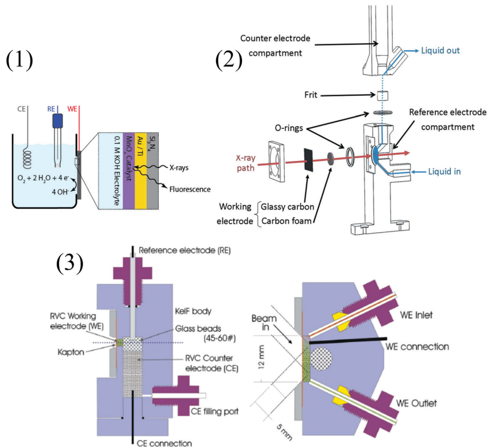
Fig. 10 Examples of XAS-SEC cells. (1) In situ XAS setup, with the back side of the \text{Si}_3\text{N}_4 window facing the X-rays and the front side of the window covered with electrodeposited MnOx on a layer of Au/Ti facing the electrolyte. CE, RE, and WE stand for counter, reference, and working electrodes, respectively; reprinted with permission from ref. 69, copyright (2013) American Chemical Society. (2) Detailed view of a spectroelectrochemical cell developed for time-resolved data collection in transmission mode; 70 and (3) vertical (left) and horizontal (right) sections through the working electrode chamber of a fluorescence X-ray absorption spectroscopy spectroelectrochemical (XAS-SEC) cell (RVC = reticulated vitreous carbon). Solution flow control is achieved using syringe pumps and Teflon tubing. The inlet and outlet tubes of the WE are sealed with the aid of Teflon ferrules; a flanged seal was used for the CE tubing. 71
