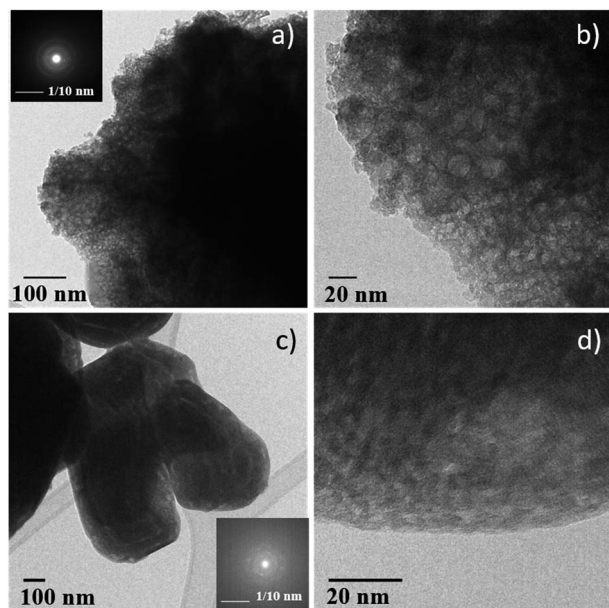
Fig. 3 TEM micrographs of (a) and (b) NiFe 2 F 4.4 O 1.8 and (c) and (d) CoFe 2 F 6.6 O 0.7 . Insets: corresponding SAED.
