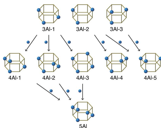
Fig. 5 Relationships between d6r species. The first row is the most abundant species in FAU; 3AI-1, 3AI-2, and 3AI-3. Arrows connect pairs of d6r species that can be transformed via isomorphic substitution between Si and Al. See Fig. S6† for complete relationships.
