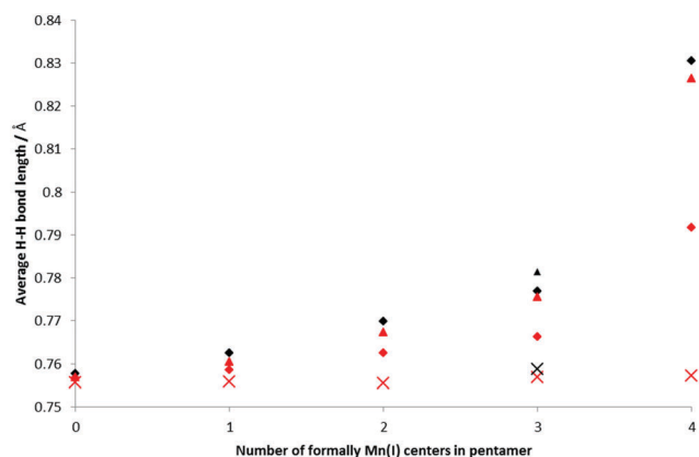
Fig. 5 Average H–H bond lengths for increasing concentrations of Mn(I). Black: 5 \text{H}_2 bound to the base structure, red: 10 \text{H}_2 , diamond: average over all, triangle: average over Kubas oriented, cross: average over non-Kubas.
