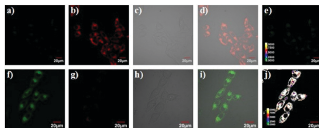
Fig. 76 Confocal fluorescence imaging without (up) and with (down) exogenous NaClO (10 \mu M) in MCF-7 cells using probe 51 (2 \mu M) for 60 min at 37 ^{\circ}\text{C} ; (a and f) green channel (500–550 nm); (b and g) red channel (655–755 nm); (c and h) bright-field images; (d and i) overlay image of (a, b and c; f, g and h); (e and j) ratio images generated from green/red channel; \lambda_{\text{ex}} = 488 nm, 635 nm. Scale bar = 20 \mu m. Copyright 2017 Elsevier.
