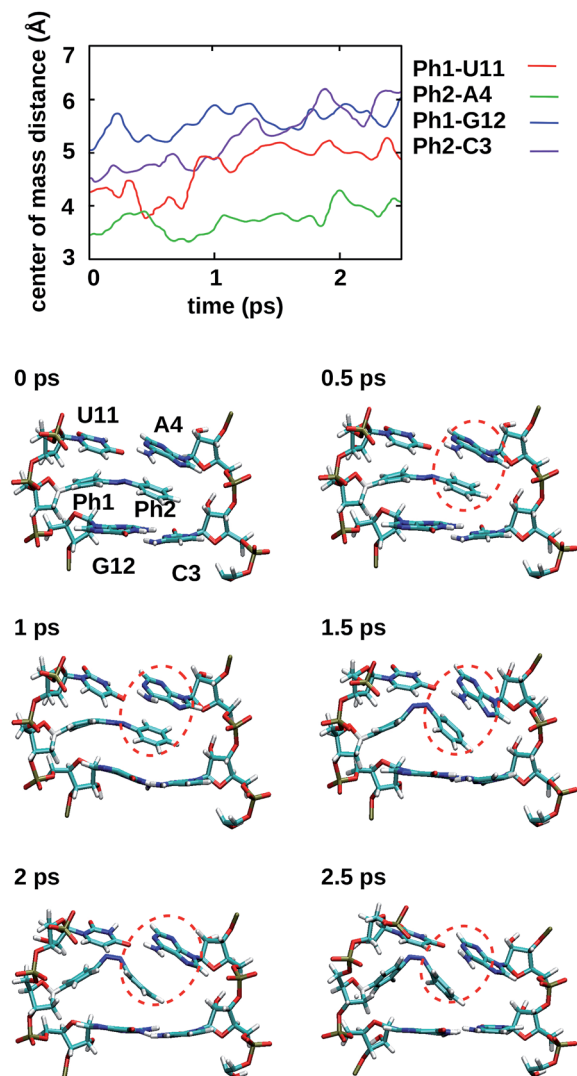
Fig. 5 For a representative trajectory taken from an Azo-RNA2 simulation, the center-of-mass distance between azobenzene and the upper and lower base pairs is shown, along with snapshots of the relevant structures for every 500 fs during the QM/MM-SH simulation. The azobenzene phenyl rings (denoted Ph1 and Ph2) are intercalated between the upper and lower bases. The snapshots show a slight decrease of stacking interactions after the switching event at \sim 1.5 ps, but stacking is preserved to a significant extent. In particular, Ph2-A4 stacking is highlighted (red circles), which persists even during and after the isomerisation event.
