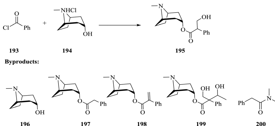
Scheme 38 Synthetic route towards Atropine.
